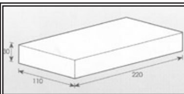
Cod. DS030350 Ladrillos porosos refractarios blancos Porous white ceramic bricks 220X110X30
