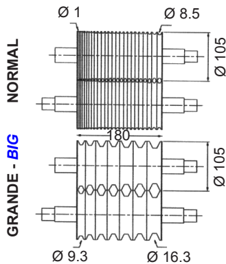
MEDIA CAÑA D-SHAPE
