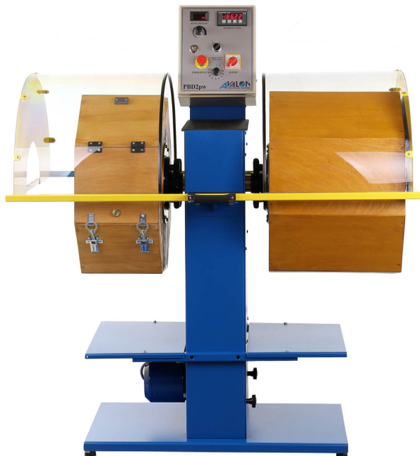
Cod. KA028060 Bombo rotativo PBD2PW Rotary Tumbler PBD2PW
