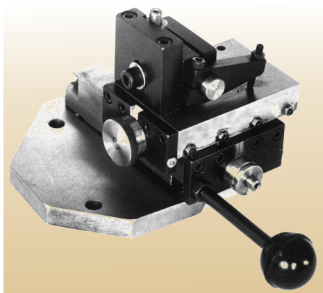
Cod. SF050406 Utillaje media caña D-shape tooling device
